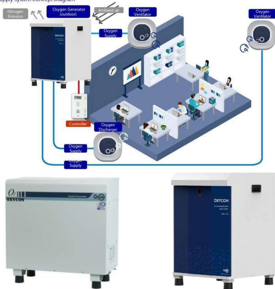
Indoor Oxygen Supply System Concept Diagram
